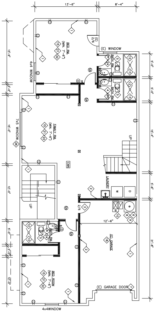
PROPOSED GROUND FLOOR PLAN SCALE: 1/4"=1'-0"
