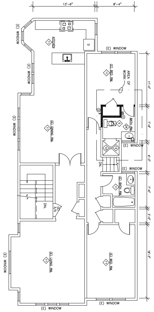
PROPOSED SECOND FLOOR PLAN SCALE: 1/4"=1'-0"
